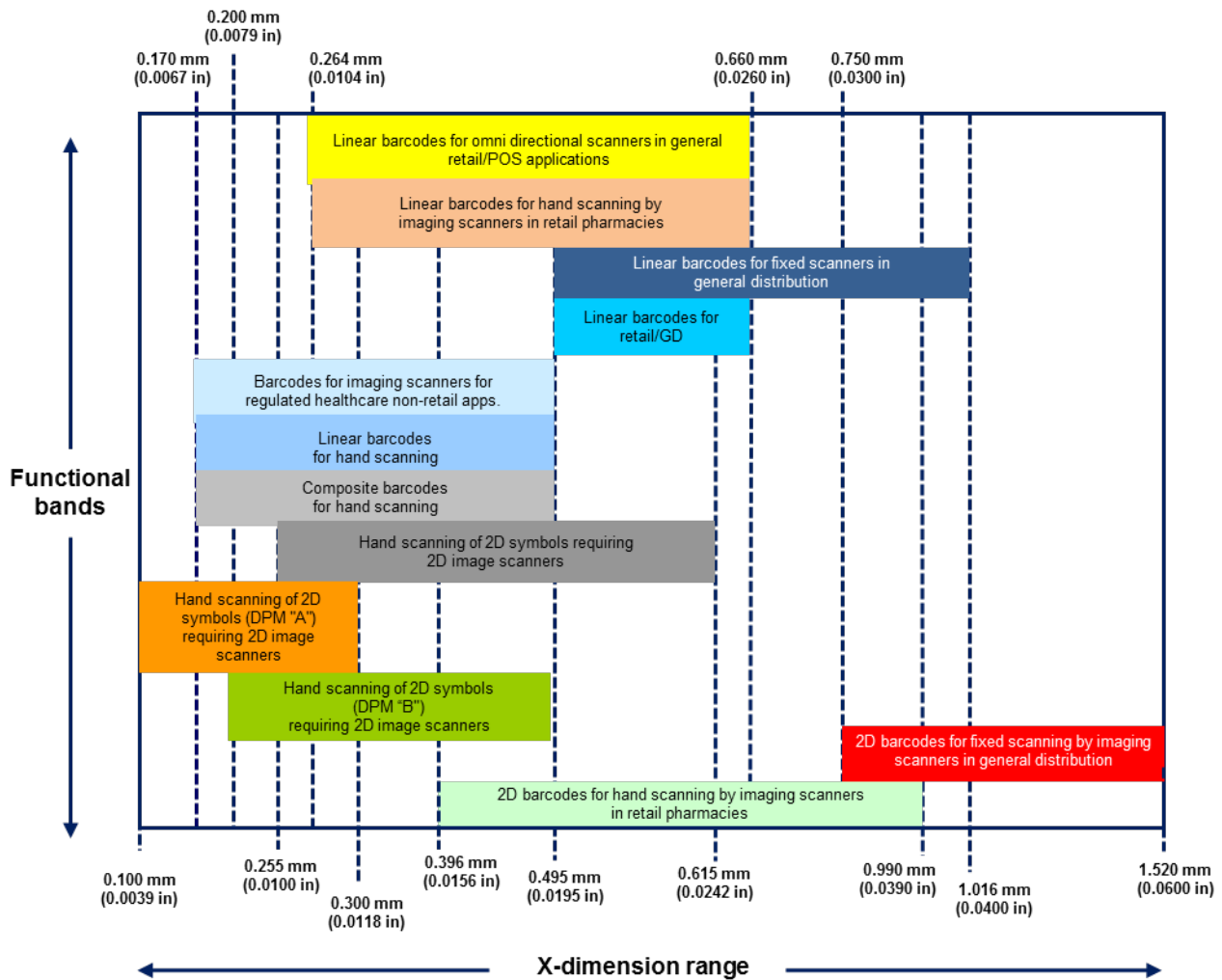
Figure 5.10.2.6-1. GS1 scanner functional operative bands
