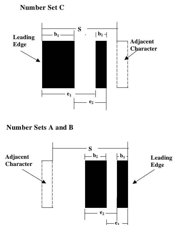
Figure 5.2.4-1. Symbol character decode measurements
